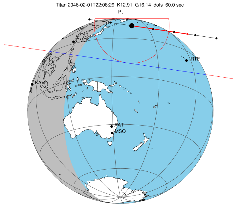
2046-02-01T22:08:29.5200 α: 17 16 34.3097 δ: -21 37 00.700 C/A 0.769" PA 8.49 deg v_sky +24.50 km/s D 10.59 AU Credit: Styled after SORA/Lucky Star
