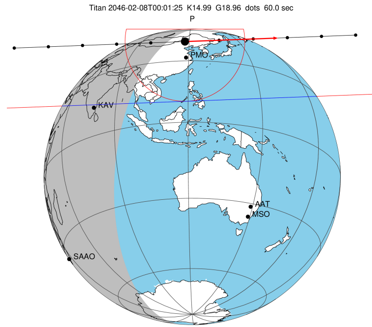
2046-02-08T00:01:25.2300 α: 17 18 23.6902 δ: -21 38 01.380 C/A 0.766" PA 357.82 deg v_sky +24.49 km/s D 10.51 AU Credit: Styled after SORA/Lucky Star
