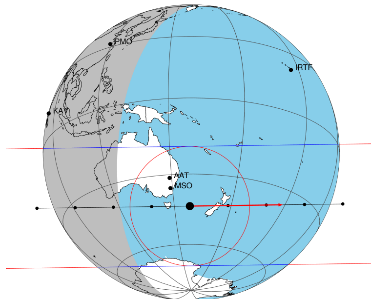
2046-02-09T21:25:27.9800 α: 17 19 03.7091 δ: -21 37 44.142 C/A 0.303" PA 179.17 deg v_sky +27.41 km/s D 10.48 AU Credit: Styled after SORA/Lucky Star
