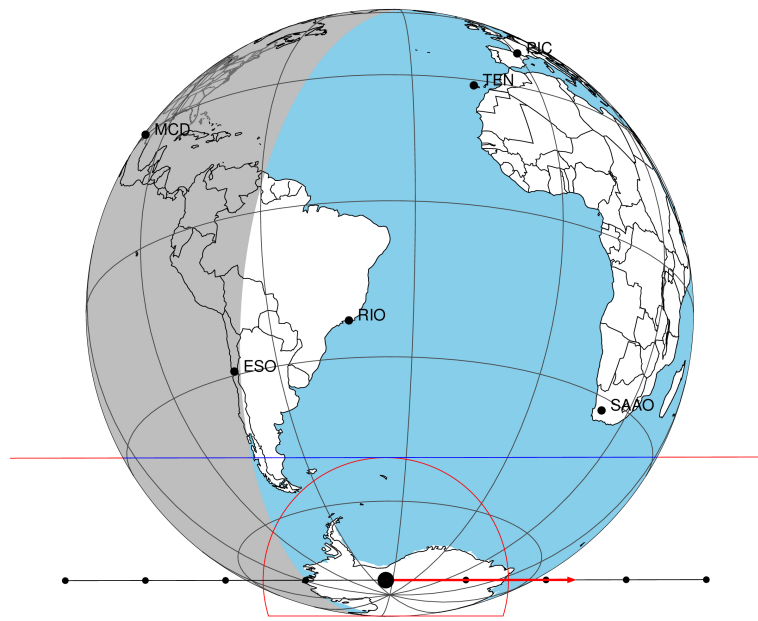
2046-02-10T10:18:31.8600 α: 17 19 15.8456 δ: -21 37 42.359 C/A 0.739" PA 179.92 deg v_sky +28.04 km/s D 10.48 AU Credit: Styled after SORA/Lucky Star
