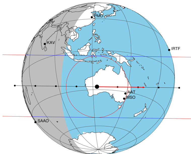
2046-02-10T23:39:09.0400 α: 17 19 28.6819 δ: -21 37 44.034 C/A 0.090" PA 180.81 deg v_sky +28.54 km/s D 10.47 AU Credit: Styled after SORA/Lucky Star
