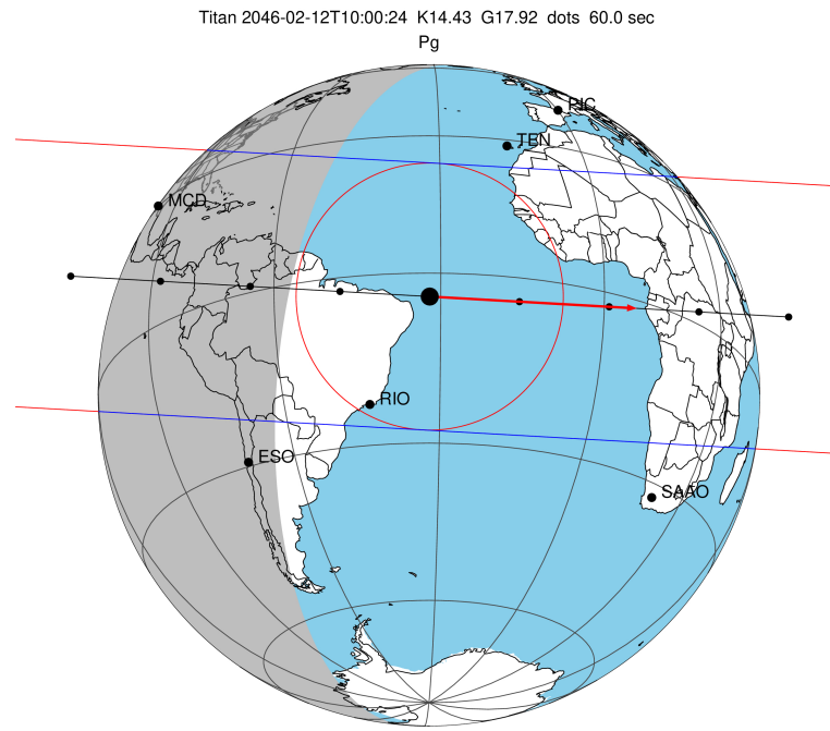
2046-02-12T10:00:24.0000 α: 17 20 02.3660 δ: -21 38 00.610 C/A 0.251" PA 3.26 deg v_sky +28.87 km/s D 10.45 AU Credit: Styled after SORA/Lucky Star
