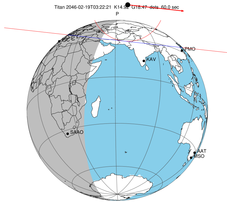
2046-02-19T03:22:21.1000 α: 17 22 08.0082 δ: -21 41 47.940 C/A 0.999" PA 6.35 deg v_sky +15.33 km/s D 10.33 AU Credit: Styled after SORA/Lucky Star
