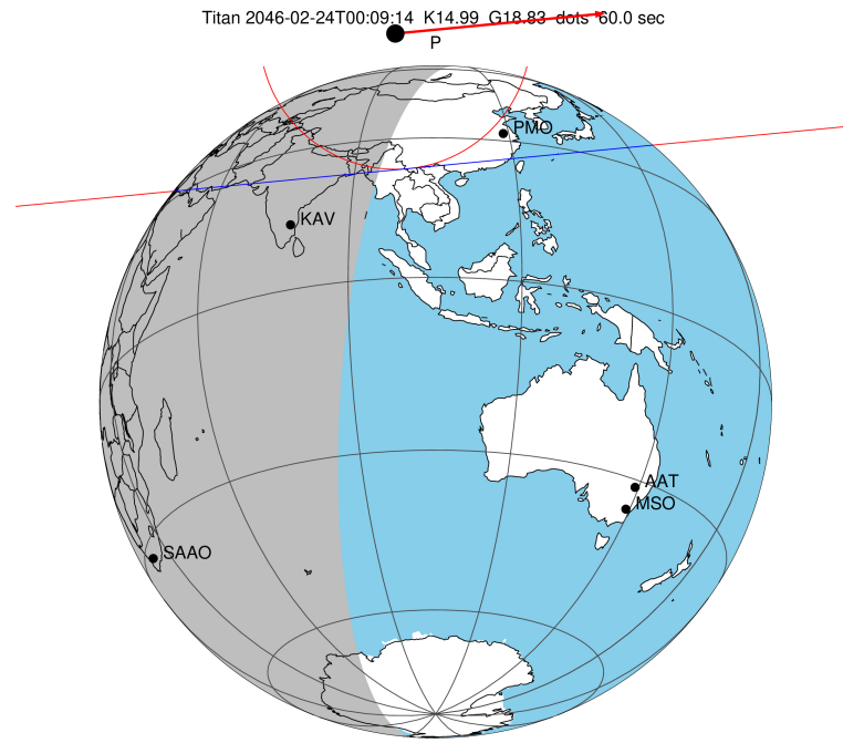
2046-02-24T00:09:14.6600 α: 17 23 08.8016 δ: -21 41 23.562 C/A 0.944" PA 354.51 deg v_sky +17.47 km/s D 10.26 AU Credit: Styled after SORA/Lucky Star
