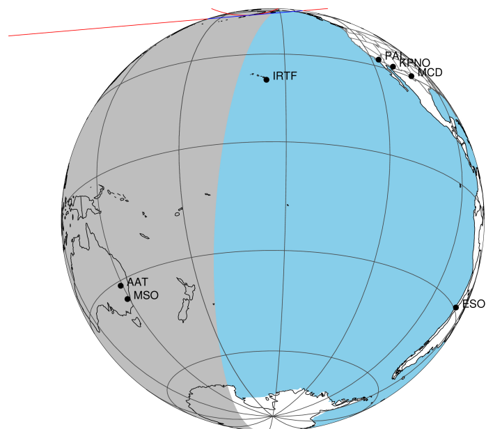
2046-02-24T17:21:32.7400 α: 17 23 19.5272 δ: -21 41 10.109 C/A 1.182" PA 355.10 deg v_sky +18.59 km/s D 10.25 AU
