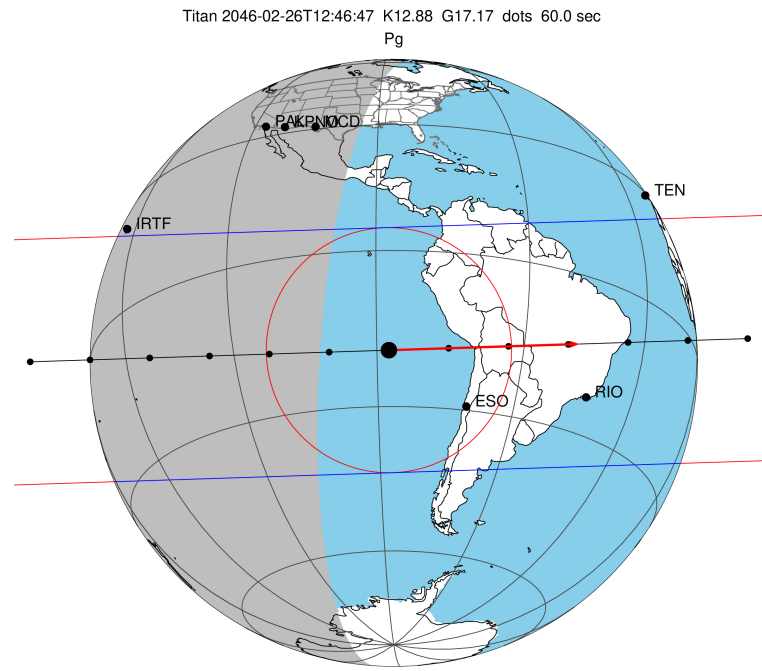
2046-02-26T12:46:47.4800 α: 17 23 49.4420 δ: -21 40 43.517 C/A 0.036" PA 358.16 deg v_sky +20.93 km/s D 10.23 AU Credit: Styled after SORA/Lucky Star
