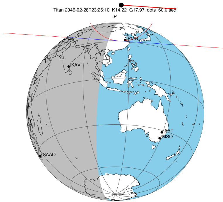
2046-02-28T23:26:10.4400 α: 17 24 33.2370 δ: -21 40 54.802 C/A 1.035" PA 3.96 deg v_sky +21.19 km/s D 10.19 AU Credit: Styled after SORA/Lucky Star
