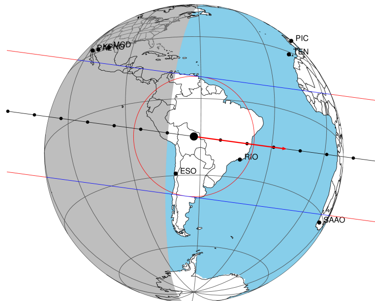
2046-03-02T10:57:03.4300 α: 17 24 58.2969 δ: -21 41 29.462 C/A 0.099" PA 7.75 deg v_sky +19.07 km/s D 10.16 AU
