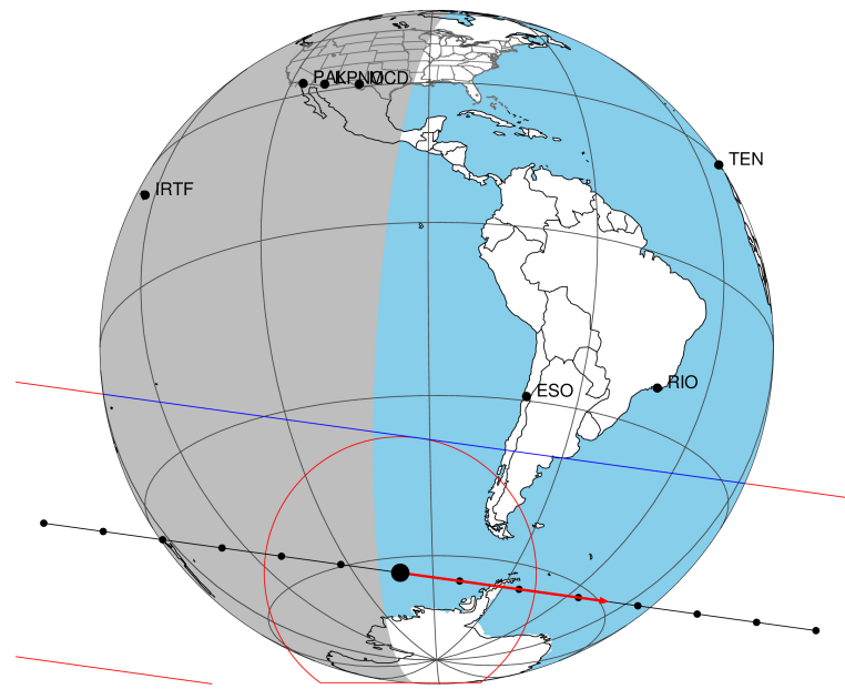
2046-03-02T12:39:53.0900 α: 17 24 59.4338 δ: -21 41 30.948 C/A 0.587" PA 187.92 deg v_sky +18.92 km/s D 10.16 AU Credit: Styled after SORA/Lucky Star
