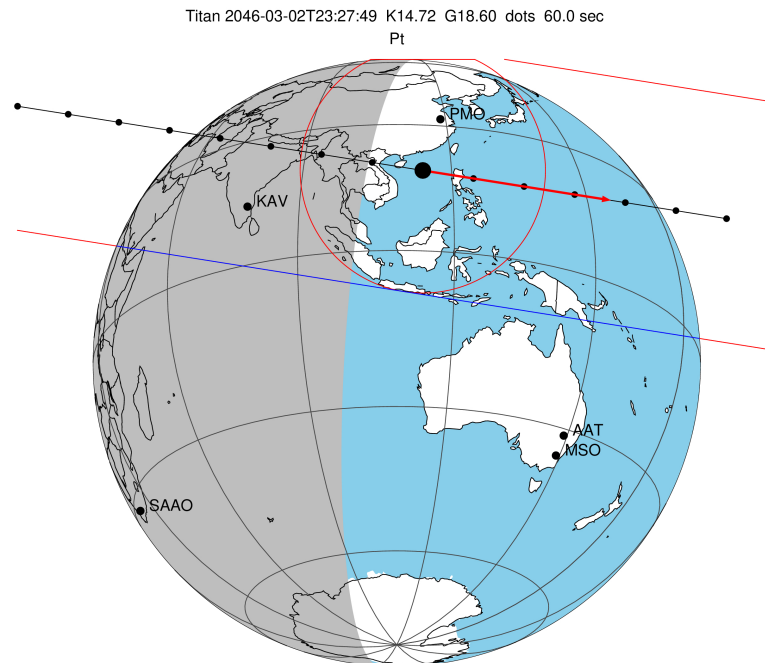
2046-03-02T23:27:49.4900 α: 17 25 06.3279 δ: -21 41 46.406 C/A 0.554" PA 9.02 deg v_sky +17.94 km/s D 10.15 AU Credit: Styled after SORA/Lucky Star
