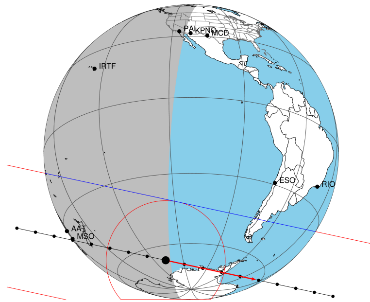
2046-03-04T14:03:20.3200 α: 17 25 27.5066 δ: -21 42 40.778 C/A 0.654" PA 192.17 deg v_sky +13.71 km/s D 10.12 AU Credit: Styled after SORA/Lucky Star
