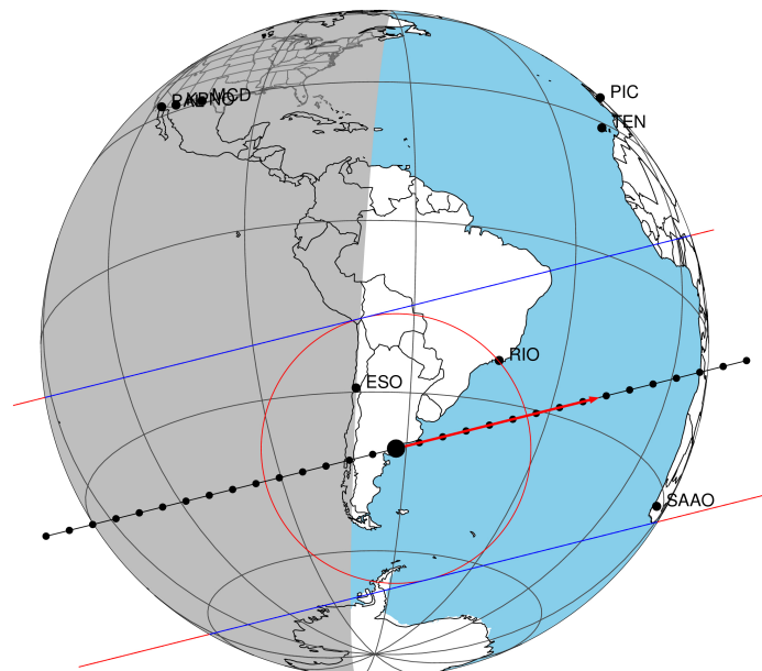
2046-03-10T10:43:58.1000 cc: 17 26 08.6293 s: -21 43 23.054 C/A 0.280" PA 165.92 deg v_sky + 7.66 km/s D 10.02 AU Credit: Styled after SORA/Lucky Star
