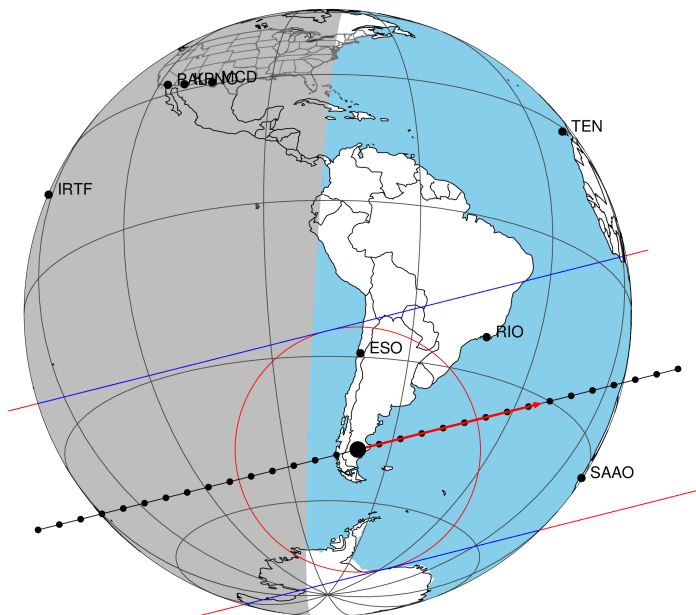
2046-03-10T11:26:45.4200 α: 17 26 08.8159 δ: -21 43 22.272 C/A 0.404" PA 165.87 deg v_sky + 7.70 km/s D 10.02 AU Credit: Styled after SORA/Lucky Star
