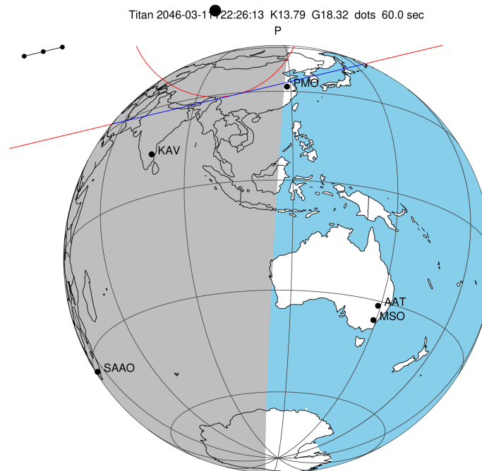
2046-03-11T22:26:13.0500 α: 17 26 19.3259 δ: -21 42 46.705 C/A 1.054" PA 346.57 deg v_sky + 9.75 km/s D 10.00 AU
