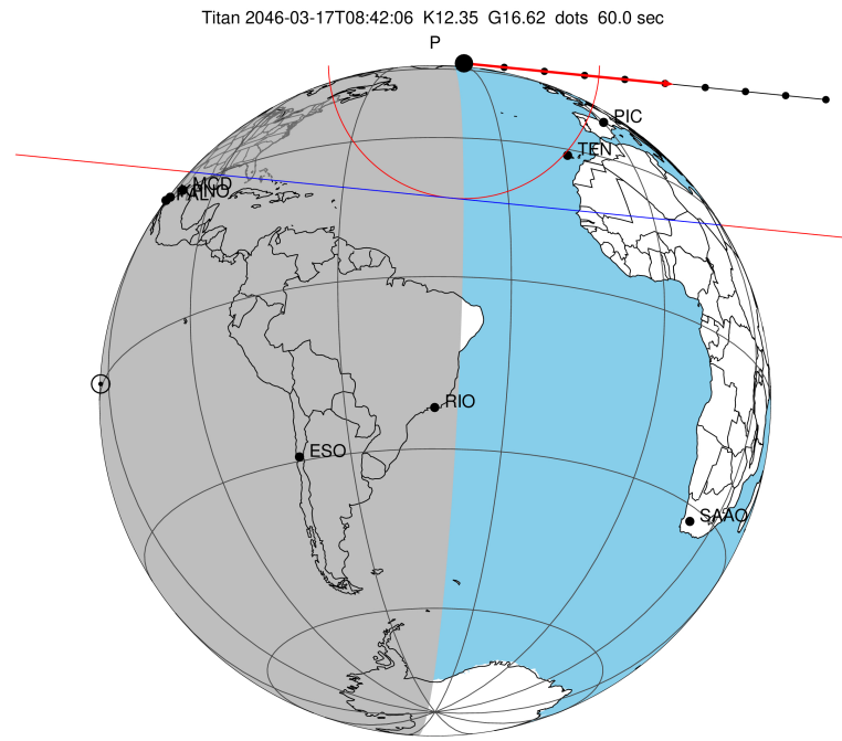
2046-03-17T08:42:06.8200 α: 17 27 17.3108 δ: -21 41 47.427 C/A 0.895" PA 5.73 deg v_sky +12.80 km/s D 09.92 AU Credit: Styled after SORA/Lucky Star
