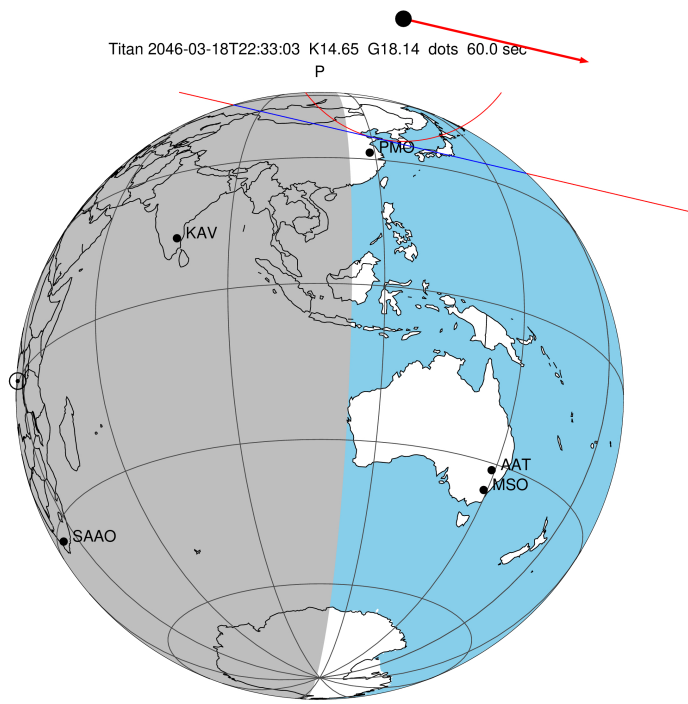
2046-03-18T22:33:03.8200 cc: 17 27 32.8203 s: -21 42 22.544 C/A 1.131" PA 13.16 deg v_sky +10.03 km/s D 09.89 AU Credit: Styled after SORA/Lucky Star
