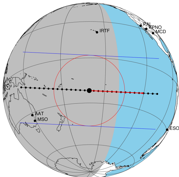
2046-04-01T15:29:45.4300 α: 17 28 04.0258 δ: -21 40 55.350 C/A 0.003" PA 182.73 deg v_sky + 5.50 km/s D 09.67 AU
