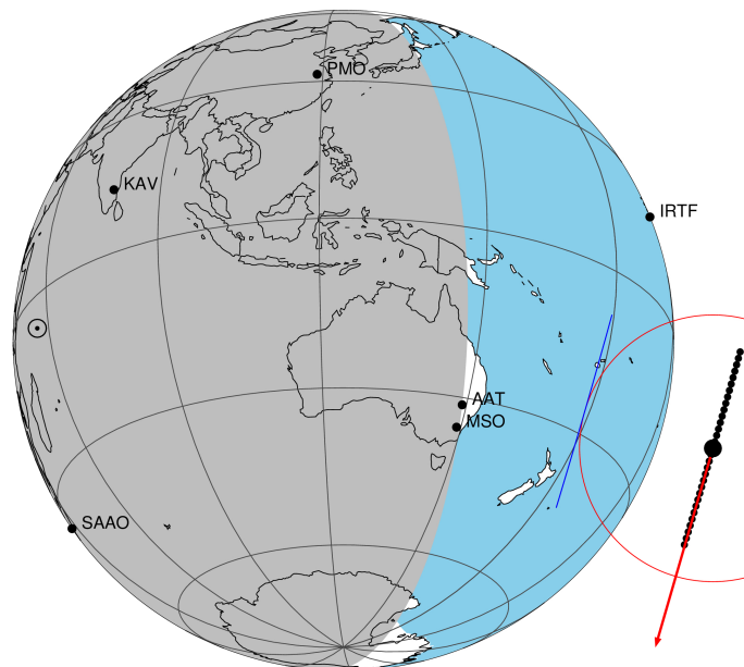
2046-04-04T20:20:45.4300 α: 17 28 12.5221 δ: -21 41 51.295 C/A 1.066" PA 106.11 deg v_sky - 2.15 km/s D 09.61 AU
