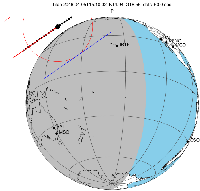
2046-04-05T15:10:02.0800 α: 17 28 11.4576 δ: -21 42 12.095 C/A 0.996" PA 325.16 deg v_sky - 3.39 km/s D 09.60 AU Credit: Styled after SORA/Lucky Star
