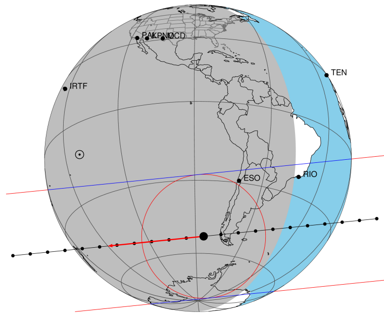
2046-04-22T09:21:17.9900 cc: 17 26 43.1786 s: -21 40 13.648 C/A 0.482" PA 174.19 deg v_sky -12.06 km/s D 09.36 AU Credit: Styled after SORA/Lucky Star
