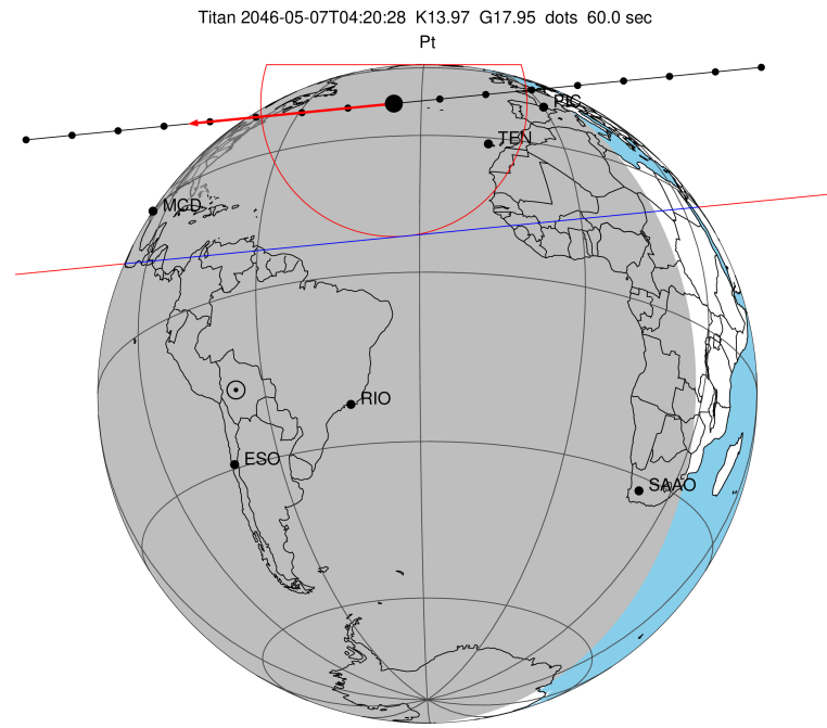
2046-05-07T04:20:28.6600 cc: 17 23 59.6934 & -21 36 42.075 C/A 0.848" PA 354.36 deg v_sky -14.89 km/s D 09.19 AU Credit: Styled after SORA/Lucky Star
