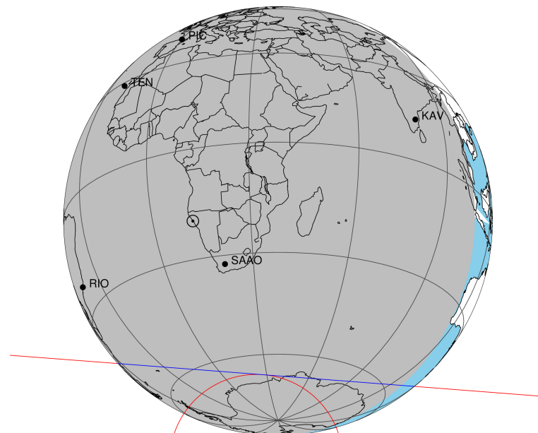
2046-05-18T23:04:53.9200 cc: 17 20 46.8016 s: -21 32 09.676 C/A 1.086" PA 184.41 deg v_sky -12.22 km/s D 09.10 AU Credit: Styled after SORA/Lucky Star
