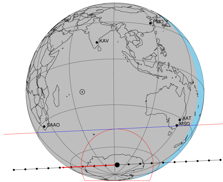
2046-05-20T19:25:10.8800 α: 17 20 24.7780 δ: -21 32 07.636 C/A 0.796" PA 177.23 deg v_sky -13.71 km/s D 09.09 AU Credit: Styled after SORA/Lucky Star
