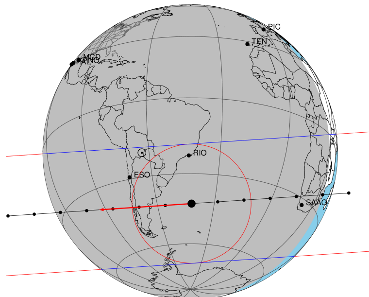
2046-05-23T04:09:10.1900 cc: 17 19 48.9818 s: -21 32 43.808 C/A 0.339" PA 176.15 deg v_sky -18.93 km/s D 09.07 AU Credit: Styled after SORA/Lucky Star
