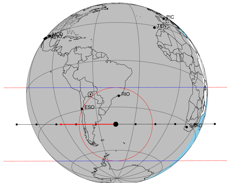
2046-05-25T04:07:42.3700 cc: 17 19 09.0431 & -21 33 04.255 C/A 0.326" PA 179.86 deg v_sky -23.21 km/s D 09.05 AU Credit: Styled after SORA/Lucky Star
