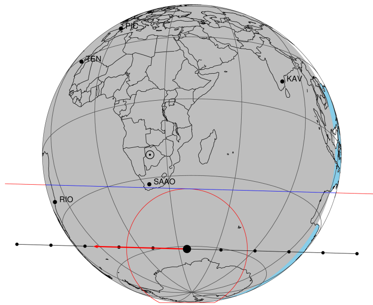
2046-05-25T22:24:52.8900 cc: 17 18 51.9835 s: -21 33 00.960 C/A 0.622" PA 181.58 deg v_sky -24.19 km/s D 09.05 AU Credit: Styled after SORA/Lucky Star
