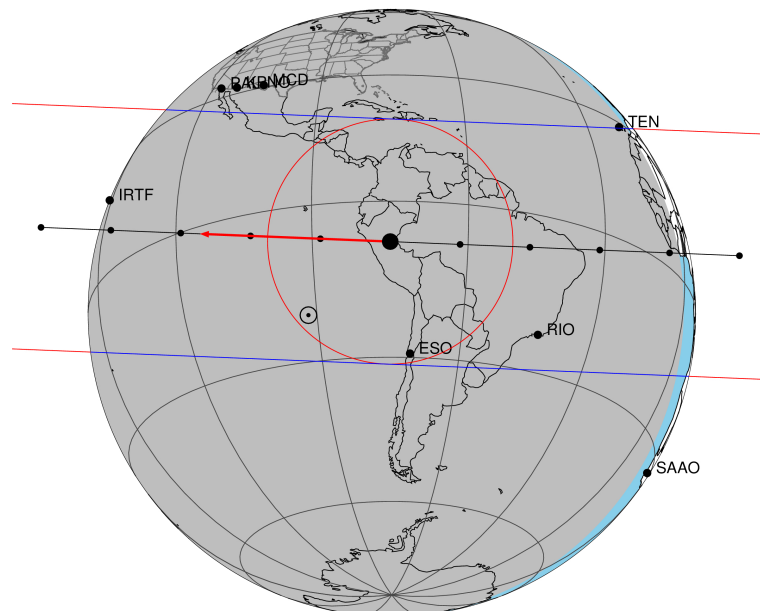
2046-05-26T06:04:12.3200 a: 17 18 44.6617 δ: -21 32 58.320 C/A 0.228" PA 2.34 deg v_sky -24.46 km/s D 09.05 AU Credit: Styled after SORA/Lucky Star
