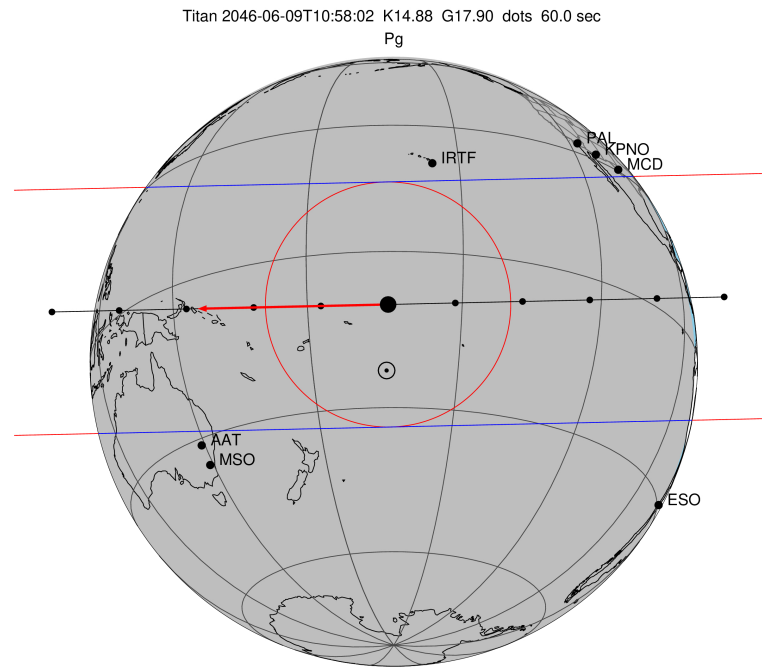
2046-06-09T10:58:02.7400 cc: 17 14 27.0910 & -21 28 34.881 C/A 0.188" PA 358.70 deg v_sky -23.53 km/s D 09.02 AU Credit: Styled after SORA/Lucky Star
