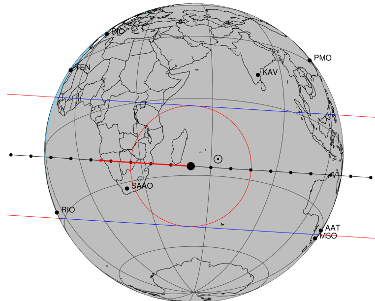
2046-06-19T19:49:47.9600 cc: 17 10 59.8046 s: -21 23 20.986 C/A 0.086" PA 183.63 deg v_sky -14.24 km/s D 09.04 AU Credit: Styled after SORA/Lucky Star
