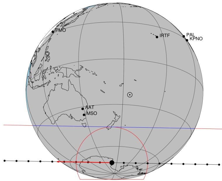
2046-06-20T11:42:31.1600 α: 17 10 50.9311 δ: -21 23 15.252 C/A 0.786" PA 181.05 deg v_sky -14.28 km/s D 09.04 AU Credit: Styled after SORA/Lucky Star
