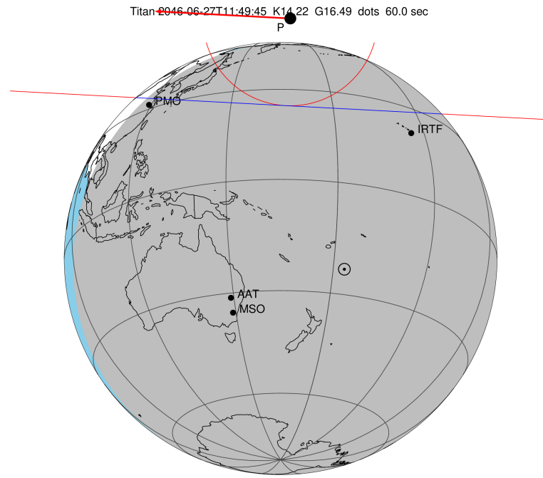
2046-06-27T11:49:45.5000 α: 17 08 41.2852 δ: -21 24 08.964 C/A 1.079" PA 3.05 deg v_sky -24.44 km/s D 09.05 AU Credit: Styled after SORA/Lucky Star
