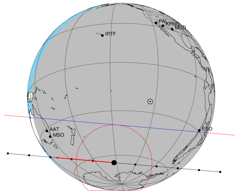
2046-06-28T08:17:31.7400 cc: 17 08 21.7979 s: -21 23 48.060 C/A 0.686" PA 184.98 deg v_sky -24.13 km/s D 09.06 AU Credit: Styled after SORA/Lucky Star
