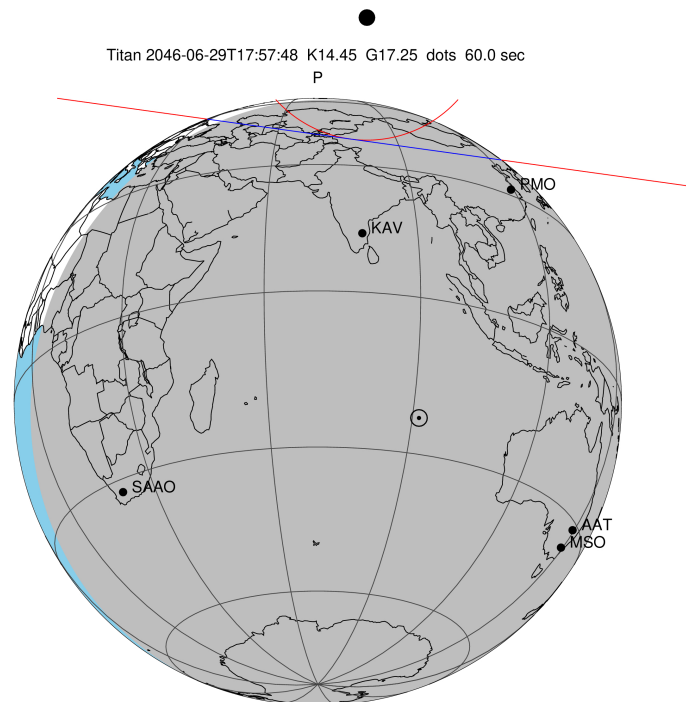
2046-06-29T17:57:48.4300 α: 17 07 51.1130 δ: -21 23 01.400 C/A 1.238" PA 7.91 deg v_sky -22.40 km/s D 09.07 AU Credit: Styled after SORA/Lucky Star
