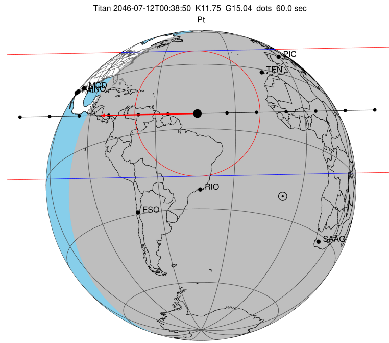
2046-07-12T00:38:50.8600 cc: 17 04 51.3468 d: -21 20 56.849 C/A 0.446" PA 358.85 deg v_sky -20.27 km/s D 09.15 AU Credit: Styled after SORA/Lucky Star
