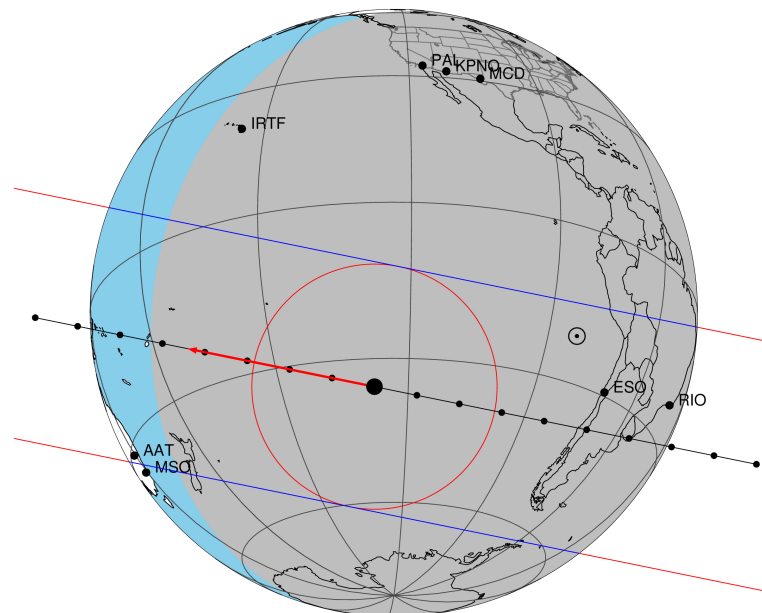
2046-07-17T05:38:30.50000 cc: 17 03 18.8415 s: -21 18 57.275 C/A 0.240" PA 191.49 deg v_sky -15.15 km/s D 09.21 AU Credit: Styled after SORA/Lucky Star
