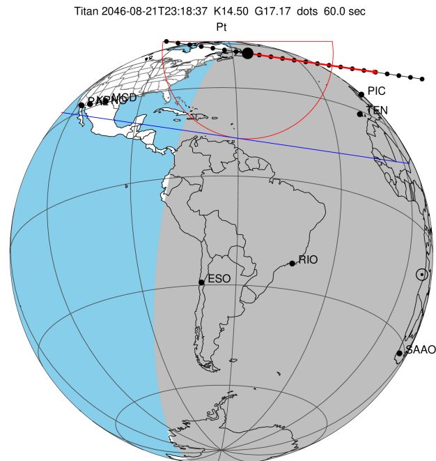
2046-08-21T23:18:37.0100 α: 16 59 31.5540 δ: -21 18 56.241 C/A 0.863" PA 8.35 deg v_sky + 5.90 km/s D 09.69 AU Credit: Styled after SORA/Lucky Star
