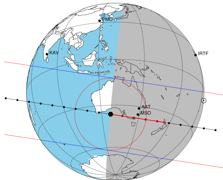
2046-09-07T09:13:23.5900 \alpha : 17 00 36.5791 \delta : -21 23 46.815 C/A 0.226" PA 188.63 deg v_sky +14.09 km/s D 09.96 AU Credit: Styled after SORA/Lucky Star
