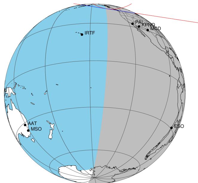
2046-09-16T03:10:48.3700 α: 17 01 51.8114 δ: -21 29 44.678 C/A 1.182" PA 8.78 deg v_sky + 7.47 km/s D 10.09 AU
