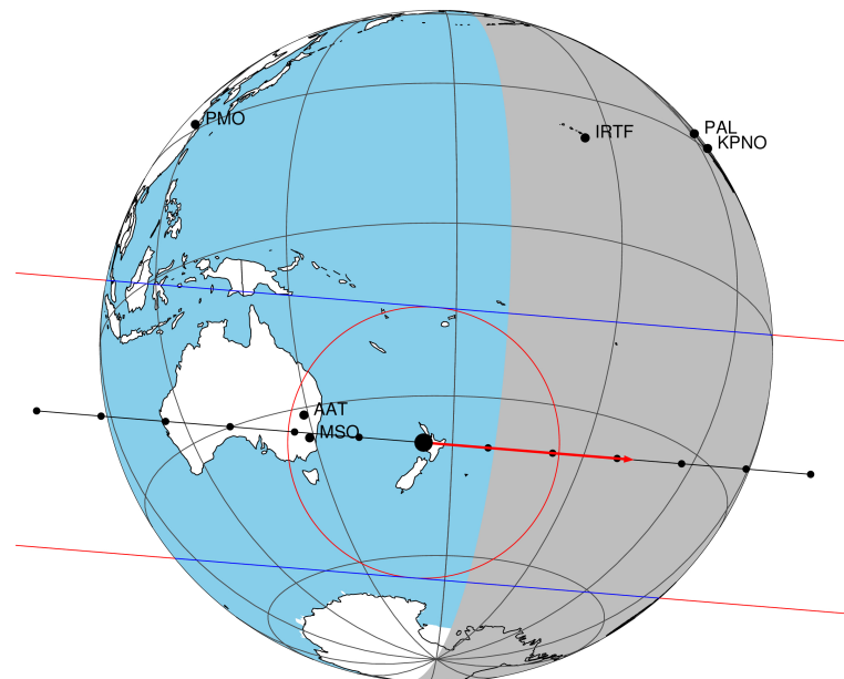
2046-09-22T05:14:57.6200 \alpha : 17 03 02.1888 \delta : -21 30 15.3500 C/A 0.248" PA 184.71 deg v_sky +20.45 km/s D 10.21 AU Credit: Styled after SORA/Lucky Star
