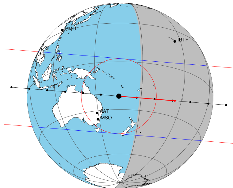
2046-09-22T05:56:56.5500 α: 17 03 02.6848 δ: -21 30 16.168 C/A 0.003" PA 185.32 deg v_sky +20.49 km/s D 10.21 AU Credit: Styled after SORA/Lucky Star
