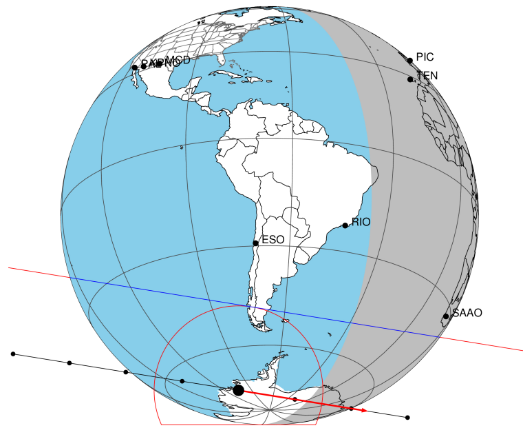
2046-10-10T20:17:52.7300 α: 17 08 17.8110 δ: -21 40 24.316 C/A 0.711" PA 189.15 deg v_sky +29.03 km/s D 10.49 AU Credit: Styled after SORA/Lucky Star
