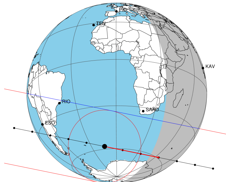
2046-10-15T15:33:13.4200 α: 17 09 55.8567 δ: -21 45 08.481 C/A 0.508" PA 191.53 deg v_sky +21.77 km/s D 10.55 AU Credit: Styled after SORA/Lucky Star
