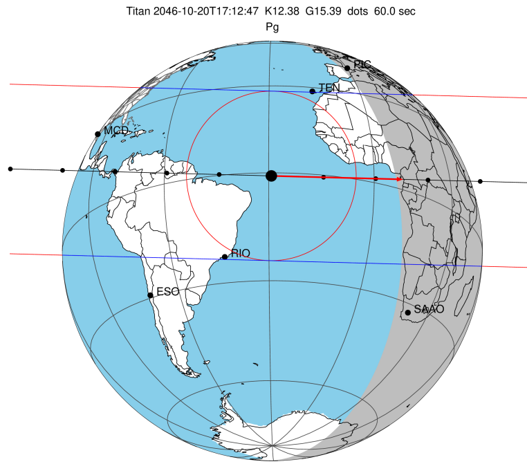
Titan 2046-10-20T17:12:47 K12.38 G15.39 dots 60.0 sec Pg 2046-10-20T17:12:47.7000 α: 17 11 27.4505 δ: -21 47 11.781 C/A 0.296" PA 1.51 deg v_sky +26.43 km/s D 10.62 AU Credit: Styled after SORA/Lucky Star
