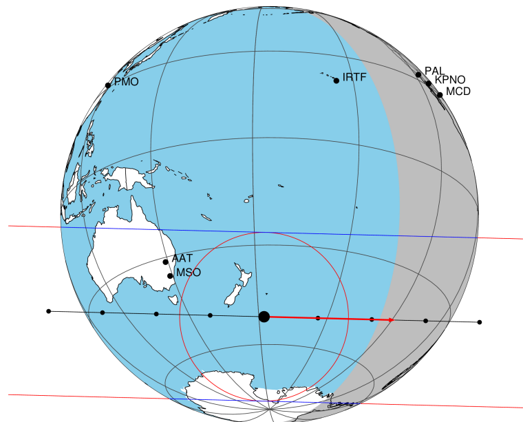
2046-10-21T02:56:37.5300 α: 17 11 36.2323 δ: -21 47 14.240 C/A 0.402" PA 181.47 deg v_sky +27.40 km/s D 10.63 AU Credit: Styled after SORA/Lucky Star
