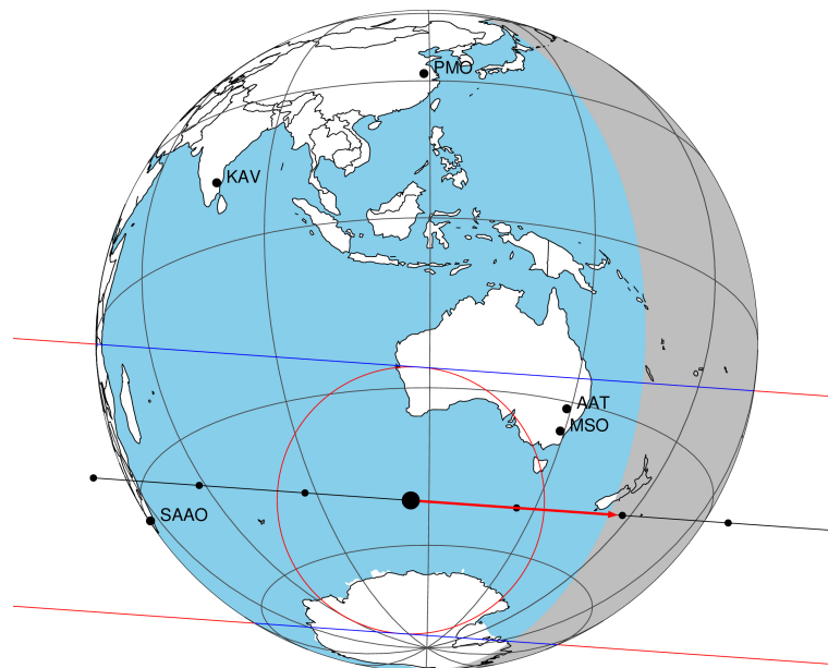
2046-10-24T07:06:29.4000 α: 17 12 55.1772 δ: -21 48 01.295 C/A 0.399" PA 184.05 deg v_sky +34.06 km/s D 10.68 AU Credit: Styled after SORA/Lucky Star
