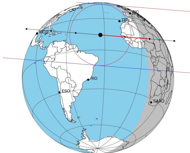
2046-10-24T17:23:27.4800 α: 17 13 06.9234 δ: -21 48 14.616 C/A 0.469" PA 4.65 deg v_sky +34.59 km/s D 10.68 AU
